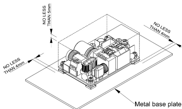
LFM200MXXXB installation diagram
