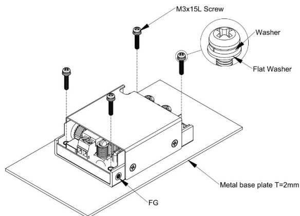
LFM200MXXXC installation diagram
