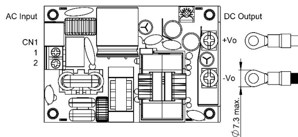
LFM200MXXB installation diagram
