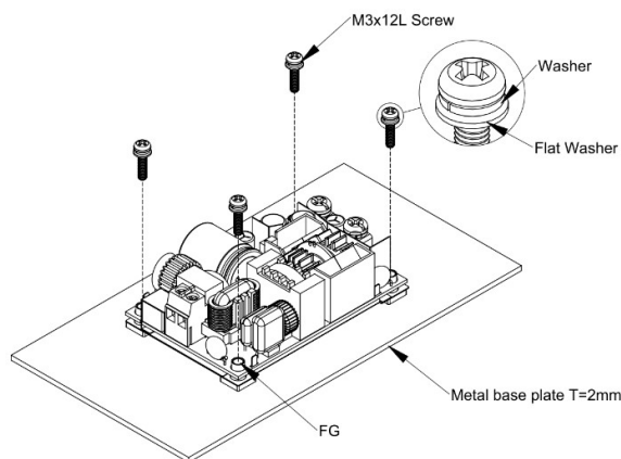
LFM200MXXXB installation diagram
