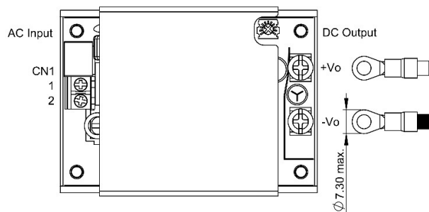
LFM200MXXC installation diagram
