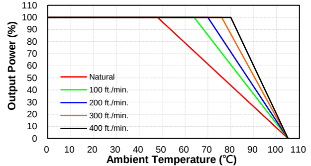
CQB75W14-72S05, 12 Derating Curve with Heatsink QBL127 (Vin=72V)
