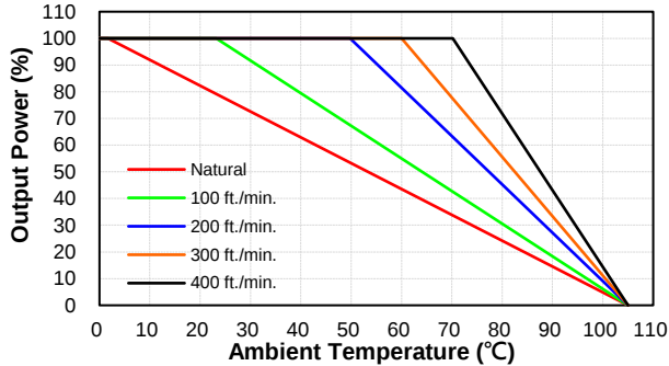
CQB75W14-72S05, 12 Derating Curve without Heatsink (Vin=72V)
