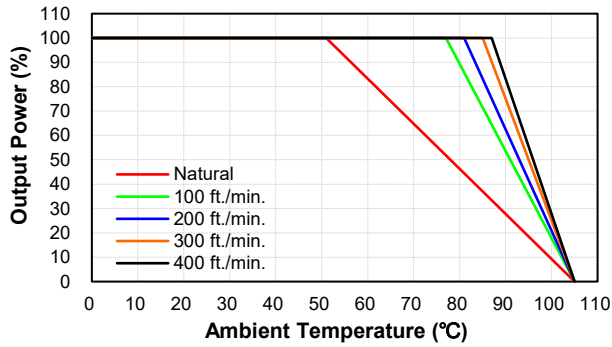
CQB100W-110S48 Derating Curve with Heatsink QBT210 (Vin=110V)
