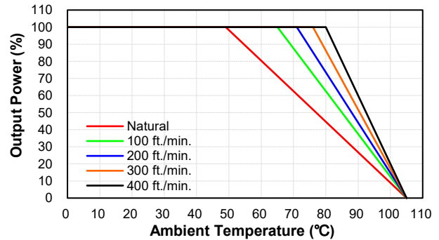
CQB100W-110S05,12,15 Derating Curve with Heatsink QBL127 (Vin=110V)
