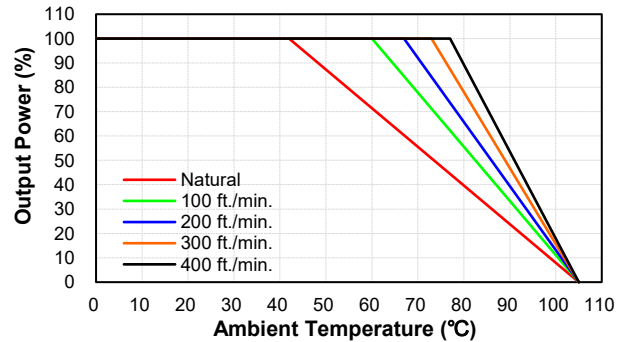
CQB100W-110S48 Derating Curve with Heatsink QBL127 (Vin=110V)
