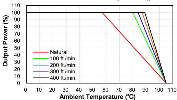
CQB100W-110S05,12,15 Derating Curve with Heatsink QBT210 (Vin=110V)
