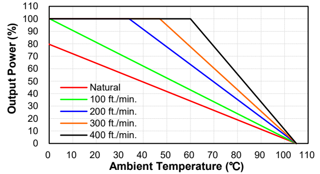
CQB100W-110S24,28 Derating Curve without Heatsink (Vin=110V)
