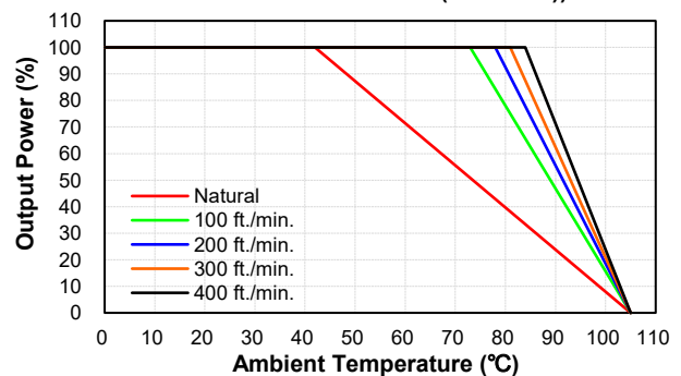
CQB100W-110S24,28 Derating Curve with Heatsink QBT210 (Vin=110V)
