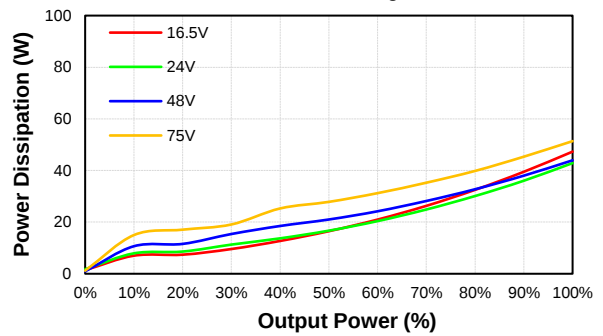
CHB500W-48S12 Pd Vs Po @25 Deg. C
