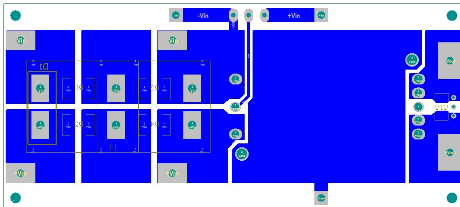
Figure4 PCB Layout Bottom View
