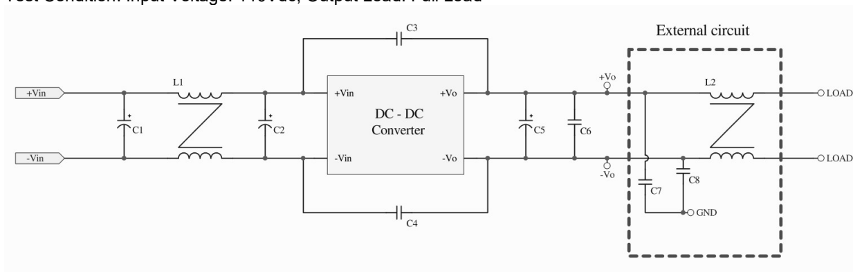
Figure2 Connection Circuit
