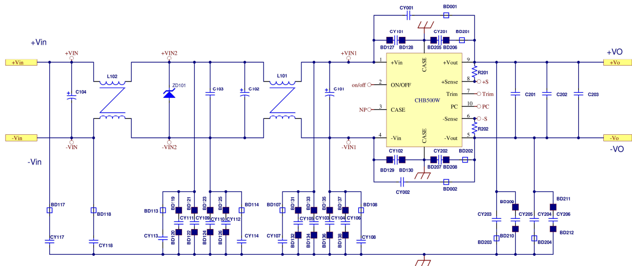
Figure1 Connection Circuit
